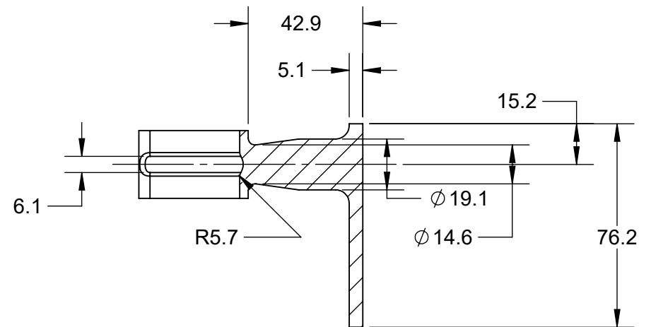
SECTION AC-AC
