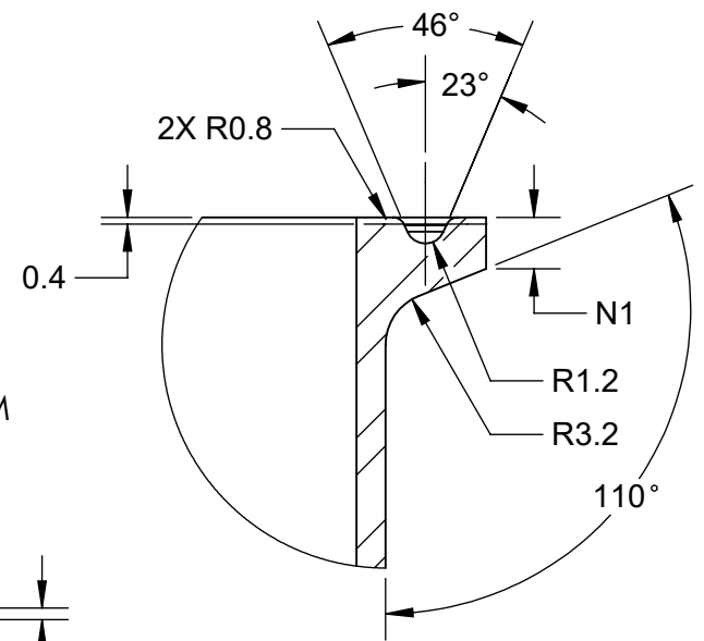
DETAIL AM SCALE 2 : 1
