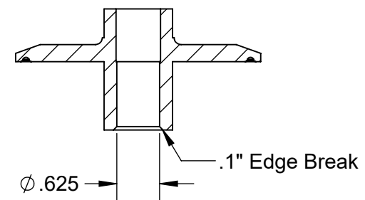
SECTION E-E
